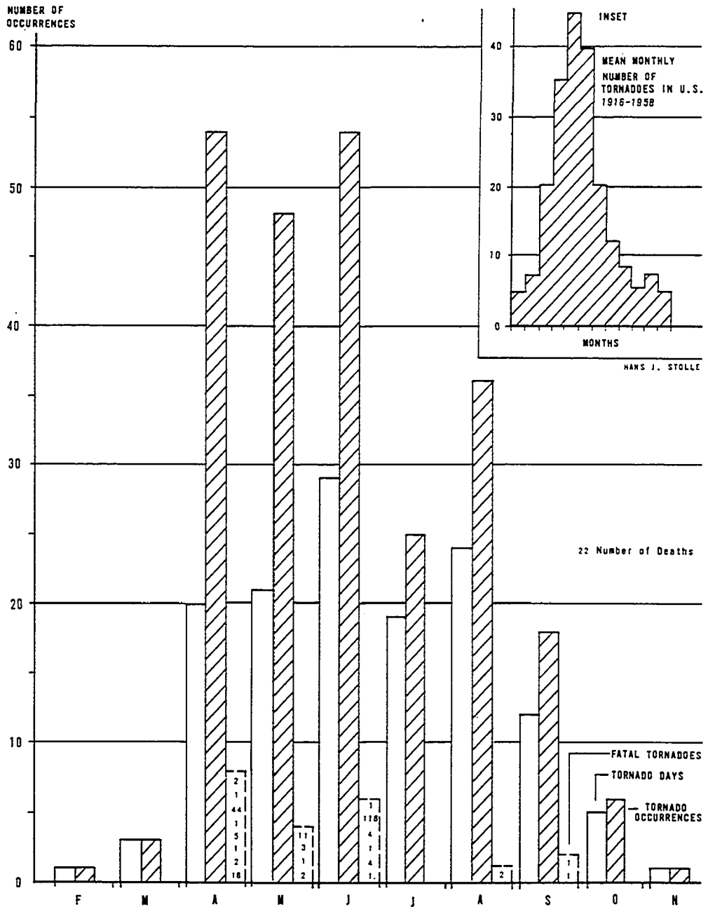
Figure 10-- FREQUENCY DISTRIBUTIONS OF TOTAL NUMBER OF MICHIGAN TORNADES, TORNADO-DAYS, AND FATAL TORNADES BY MONTHS, 1930-1969
