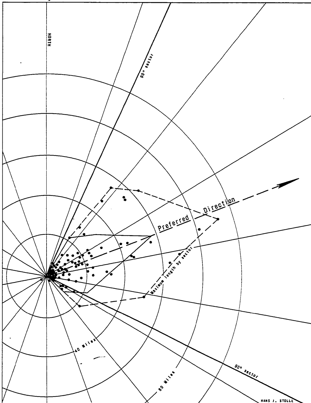
Figure 4-- PREFERRED DIRECTION OF MICHIGAN TORNAOES, 1930-1969
